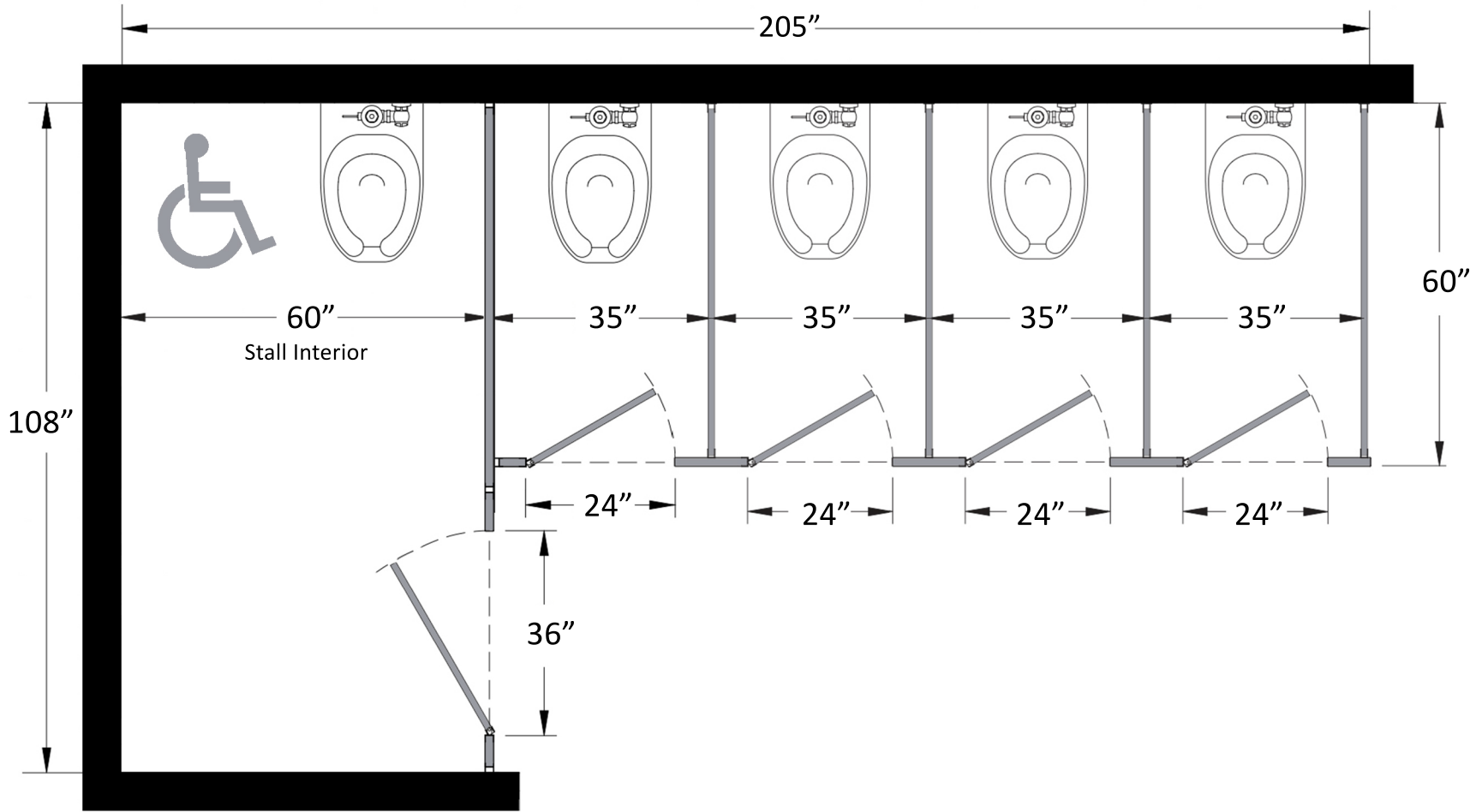
Bathroom Partitions - 5 Stall Alcove Left Hand ADA SKU: ALIC5LADA Standard Dimensions
